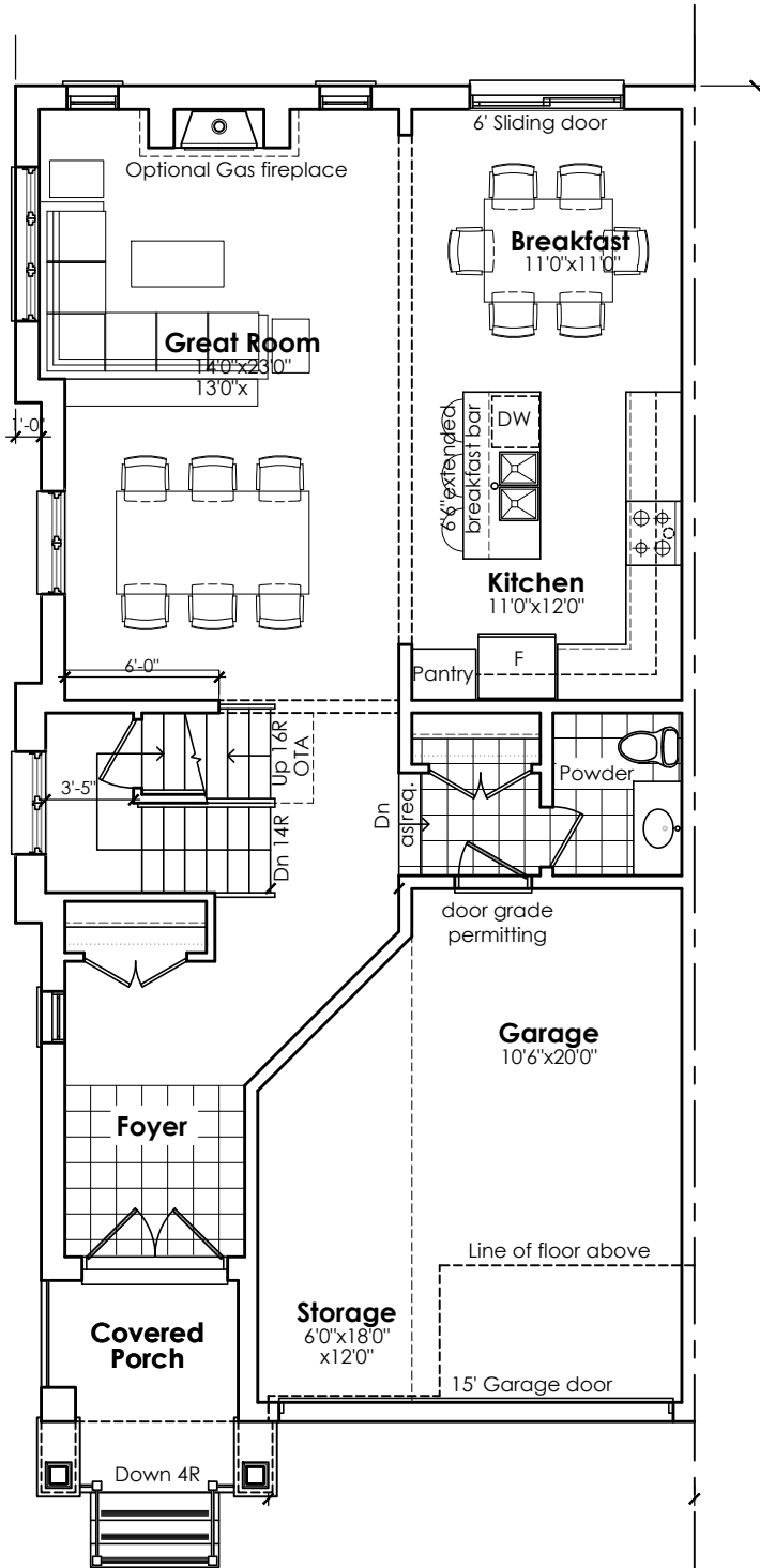
Ground Floor Plan - Corner Unit
