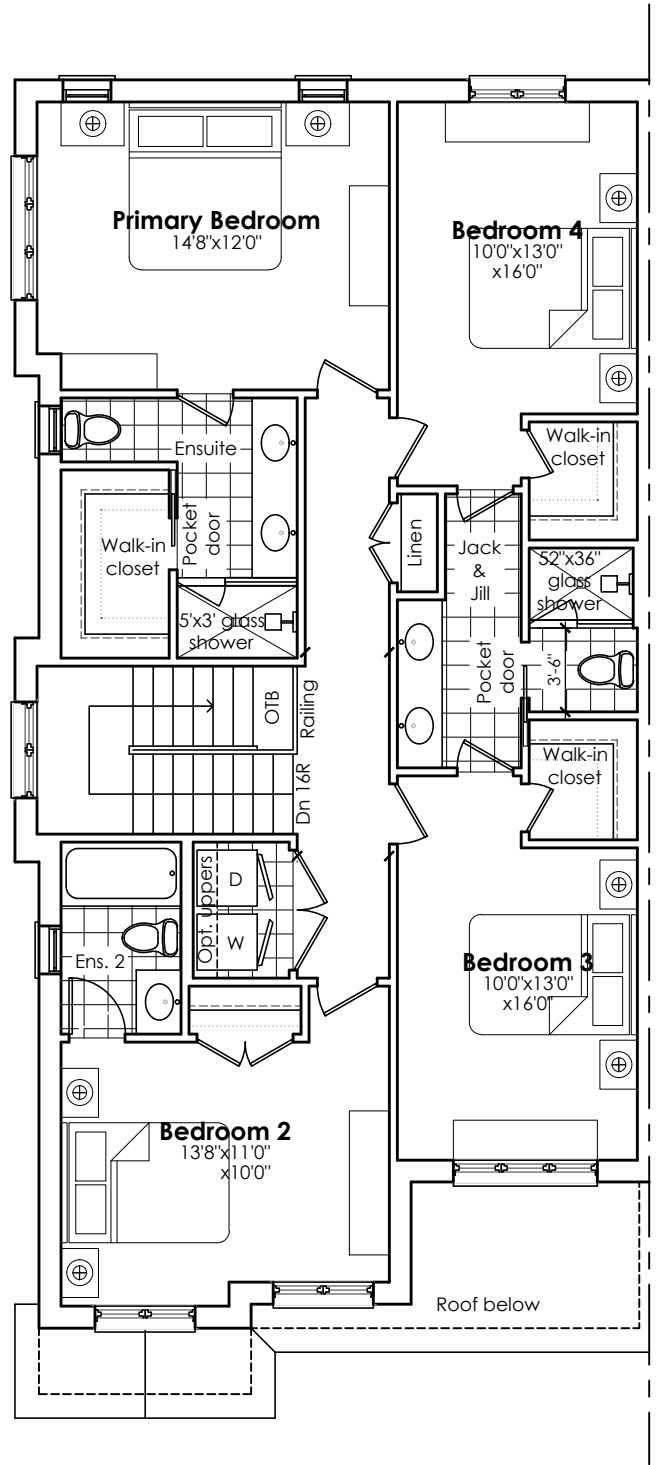
Second Floor Plan - Corner Unit
