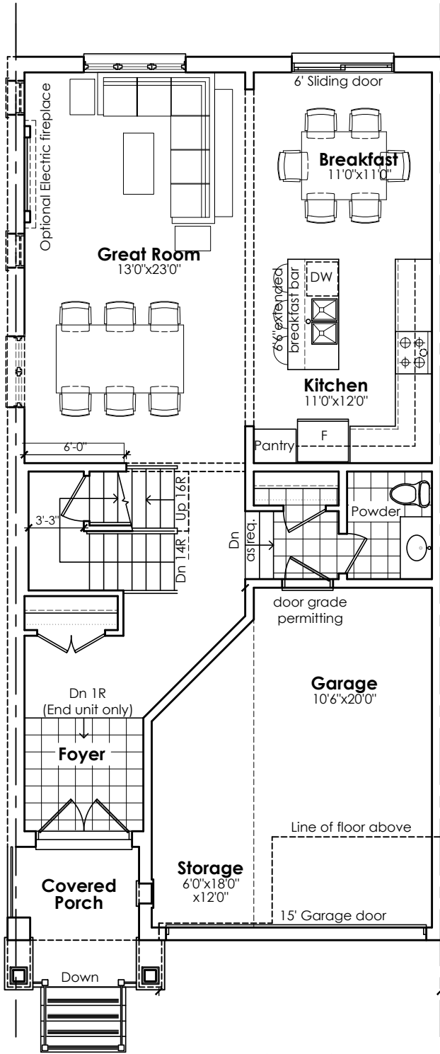
Ground Floor Plan - Interior Unit & End Unit
